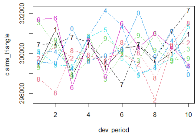
Figure 24. Plot of simulated claims triangle data.
