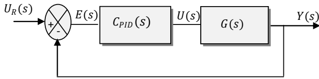
Figure 1. Feedback control loop of integer PID controller.
