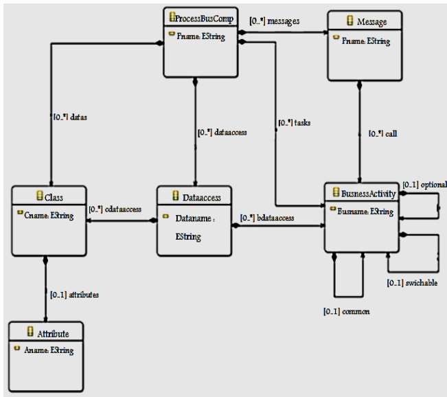
Figure 3. The business component meta-model.
