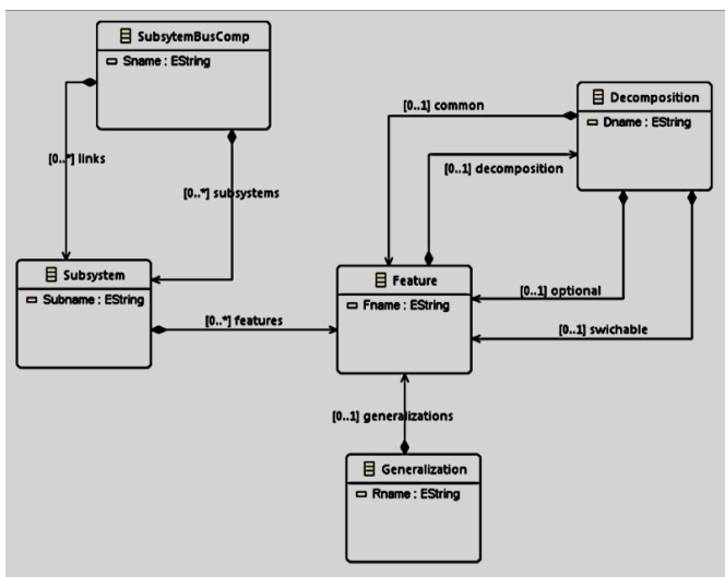
Figure 2. The meta-model of the sub-system business component.
