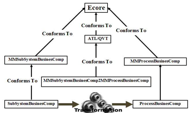
Figure 4. Subsystem model to process model transformation
